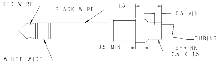
VIEW: A-A
